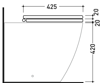
art. LK117G - LK117R vista laterale / lateral view
